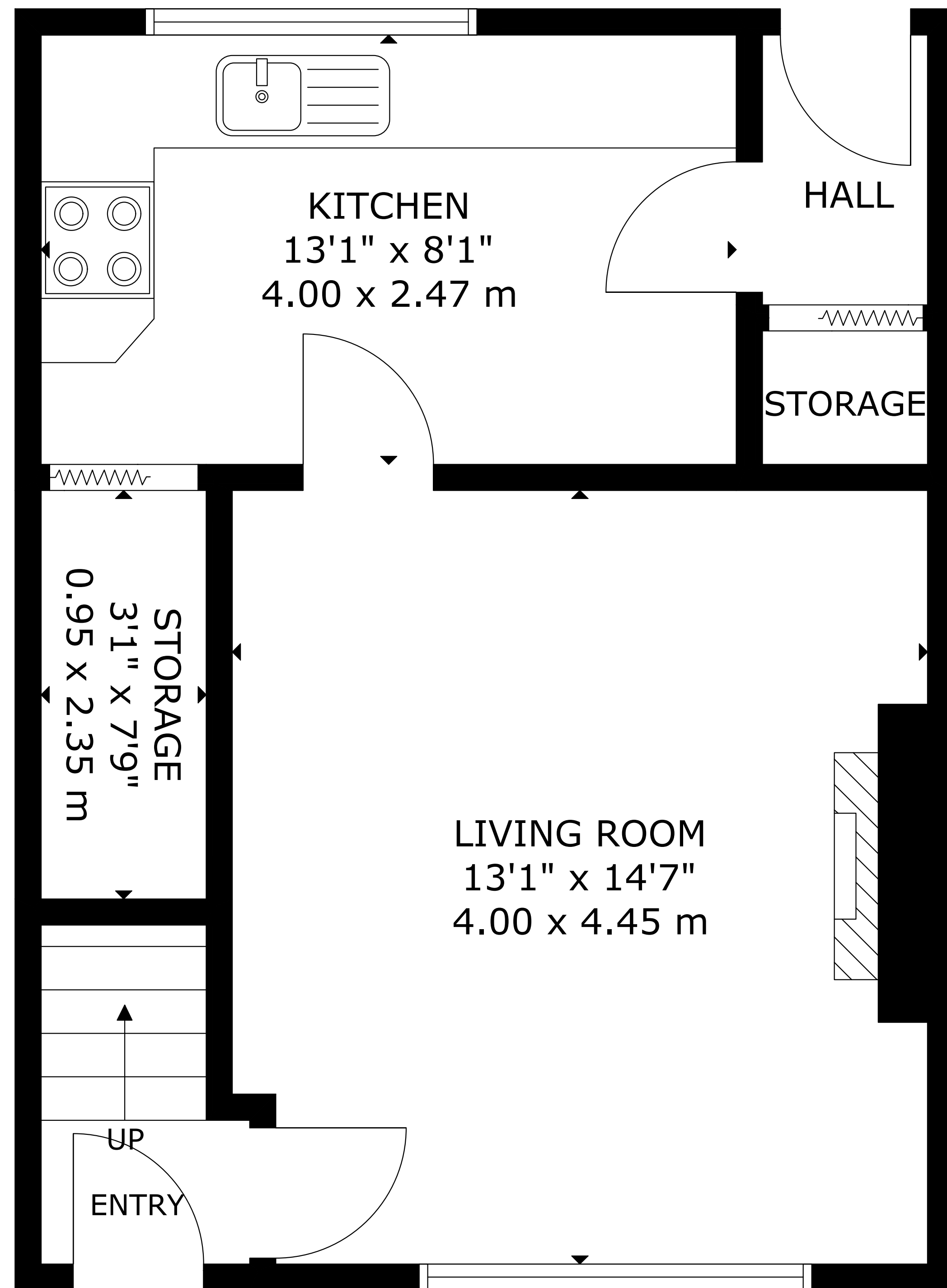
GROUND FLOOR
