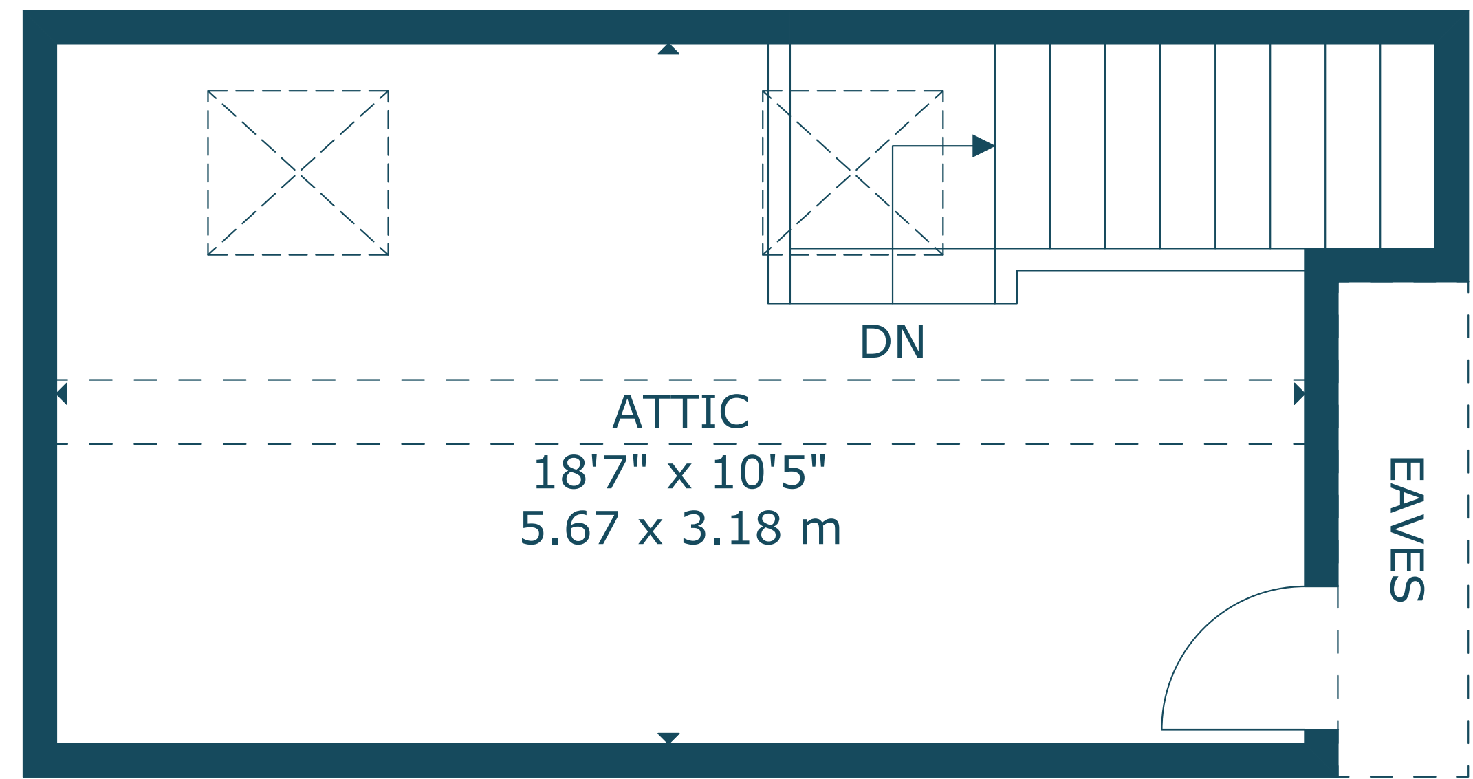
SECOND FLOOR
