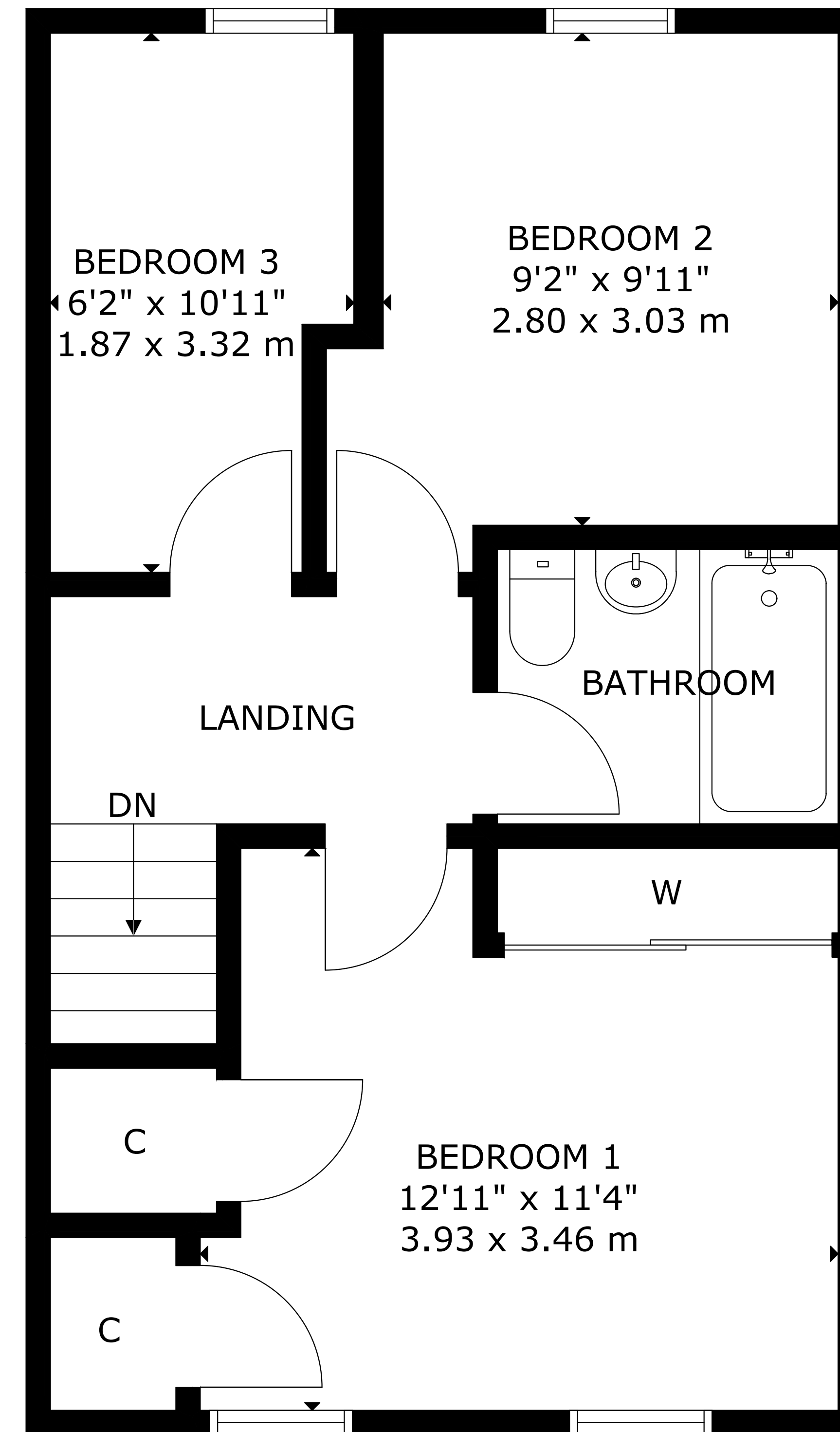
FIRST FLOOR
